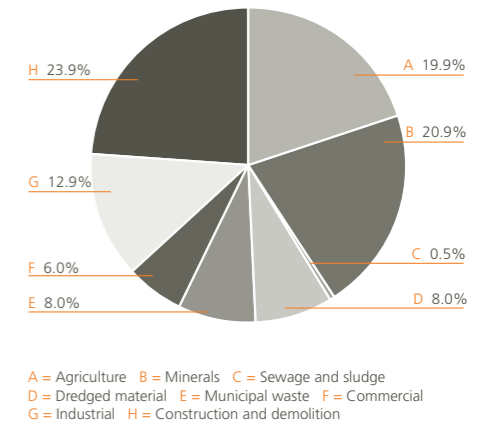
Figure 4. UK waste arisings in 2002/03 9
