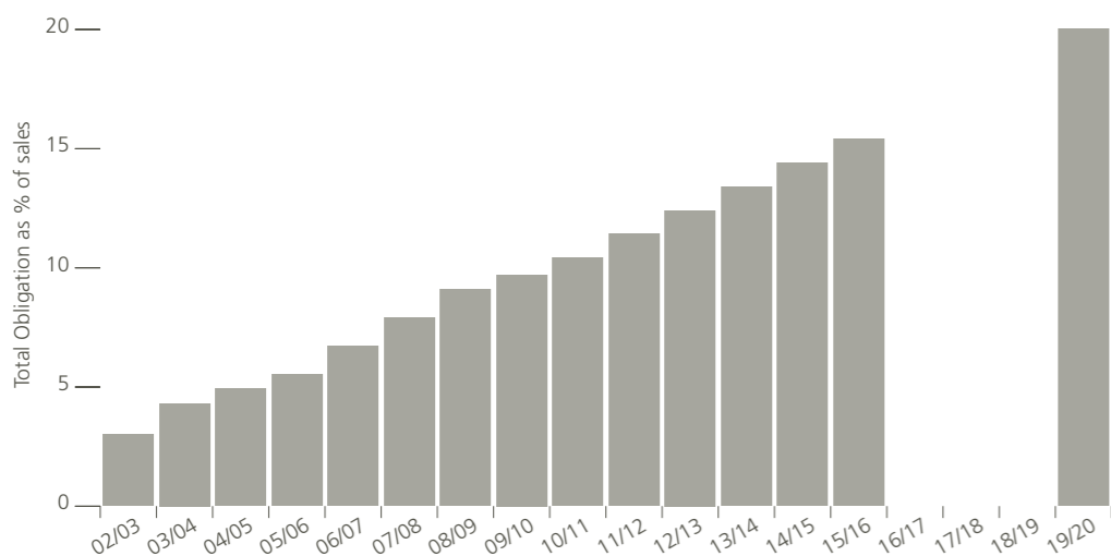
Figure 2. Renewable Obligations 2002 to 2020 ii .
