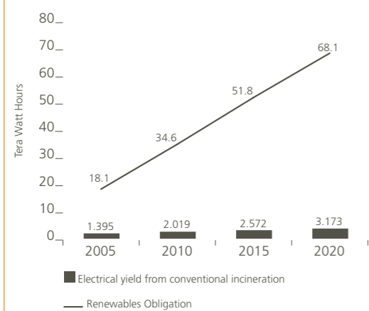
Figure 20. Potential electrical yield from conventional incineration of rBMW 2005 to 2020.
